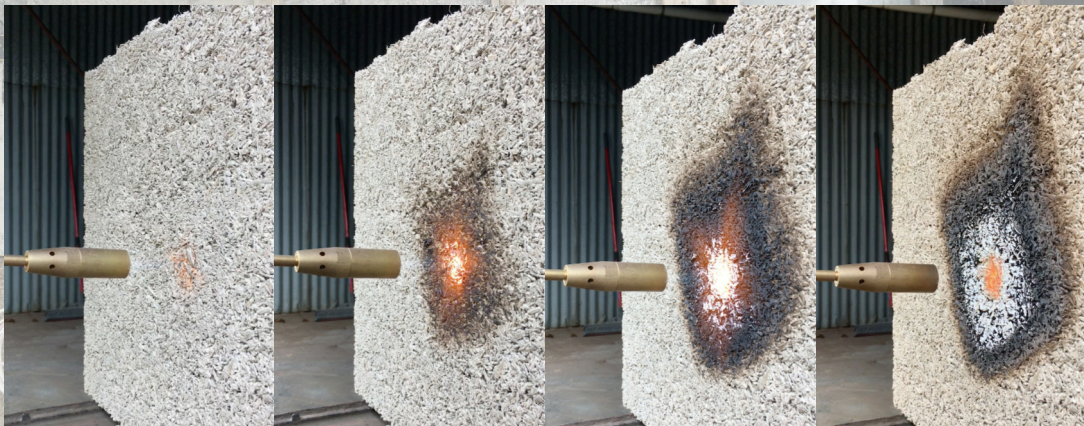
6 minute blow torch test
