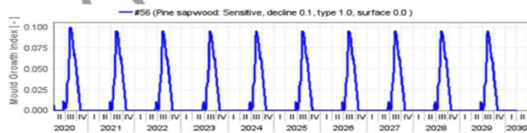
Figure 21: Timber clad wall, northern orientation, NatHERS CZ66, AS4200 Class 4 permeable building membrane (1.1403 ug/N.s)
