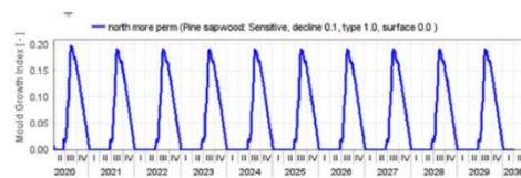
Figure 19: Timber clad wall, northern orientation, NatHERS CZ66, AS4200 Class 4 extremely permeable building membrane (not available in Australia)
