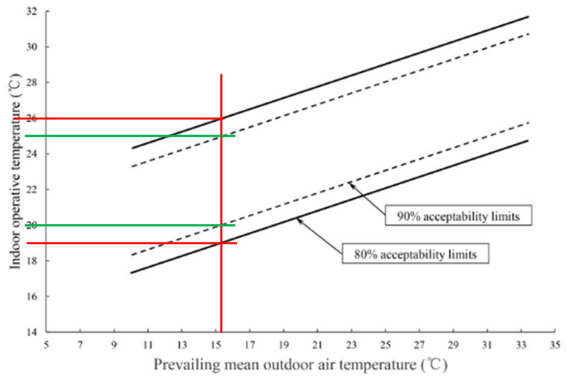
Figure 2: Adaptive comfort models represented in ANSI/ASHRAE 55:2017.
