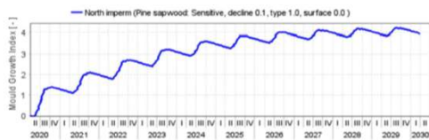
Figure 16: Timber clad wall, northern orientation, NatHERS CZ66, impermeable building membrane
