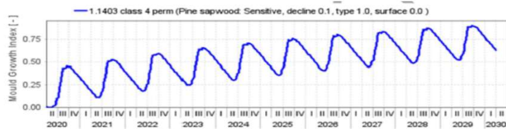
Figure 20: Timber clad wall, northern orientation, NatHERS CZ66, AS4200 Class 4 permeable building membrane (1.1403 ug/N.s)
