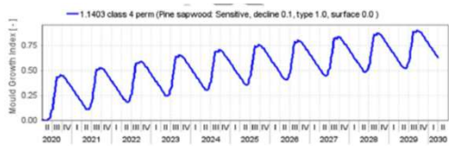
Figure 18: Timber clad wall, northern orientation, NatHERS CZ66, AS4200 Class 4 building membrane (1.1403 ug/N.s)
